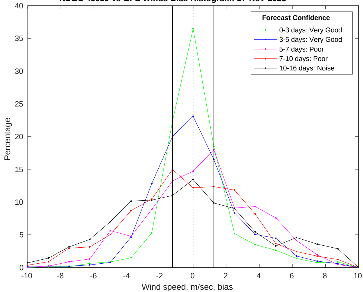
NDBC 46059 vs GFS Winds Bias Histogram: 17-Nov-2025
