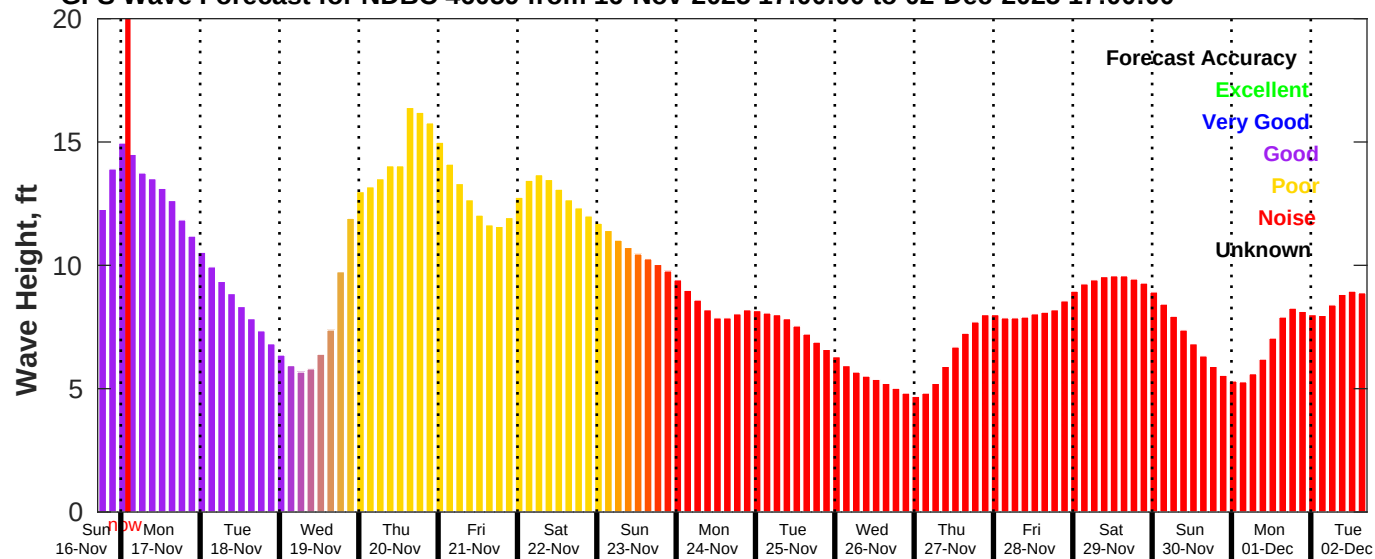
GFS Wave Forecast for NDBC 46059 from 16-Nov-2025 17:00:00 to 02-Dec-2025 17:00:00
