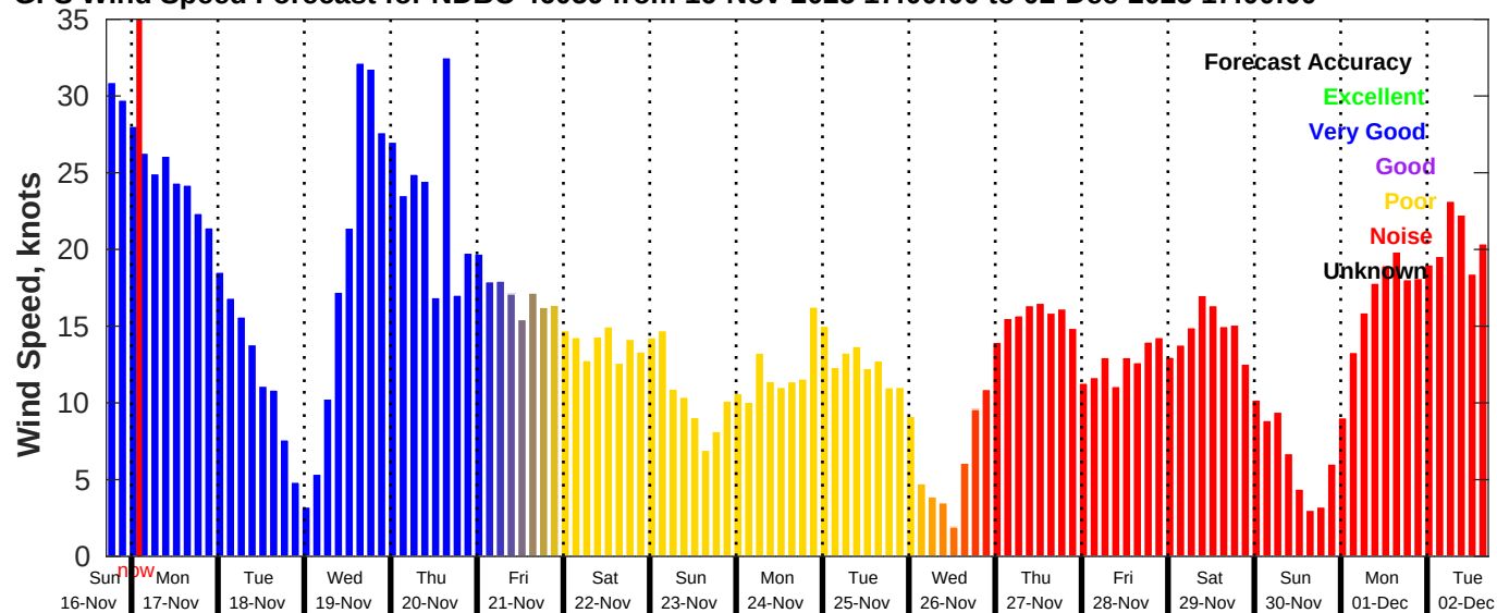
GFS Wind Speed Forecast for NDBC 46059 from 16-Nov-2025 17:00:00 to 02-Dec-2025 17:00:00
