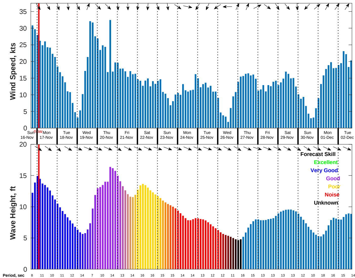
Wind & Wave Forecast for NDBC 46059 from 16-Nov-2025 17:00:00 to 02-Dec-2025 17:00:00
