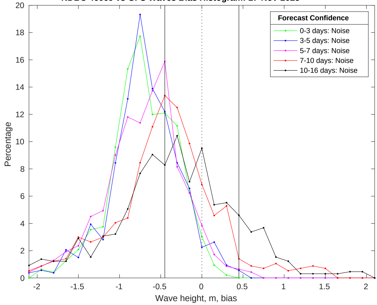
NDBC 46069 vs GFS Waves Bias Histogram: 17-Nov-2025
