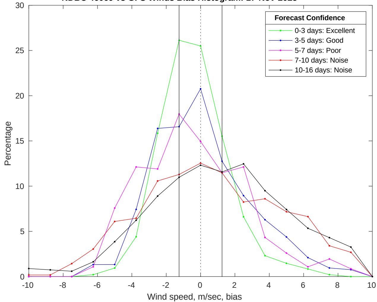
NDBC 46069 vs GFS Winds Bias Histogram: 17-Nov-2025
