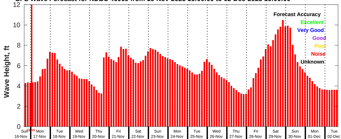
GFS Wave Forecast for NDBC 46069 from 16-Nov-2025 16:00:00 to 02-Dec-2025 16:00:00
