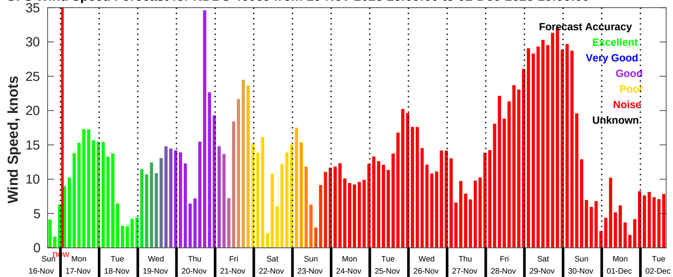
GFS Wind Speed Forecast for NDBC 46069 from 16-Nov-2025 16:00:00 to 02-Dec-2025 16:00:00
