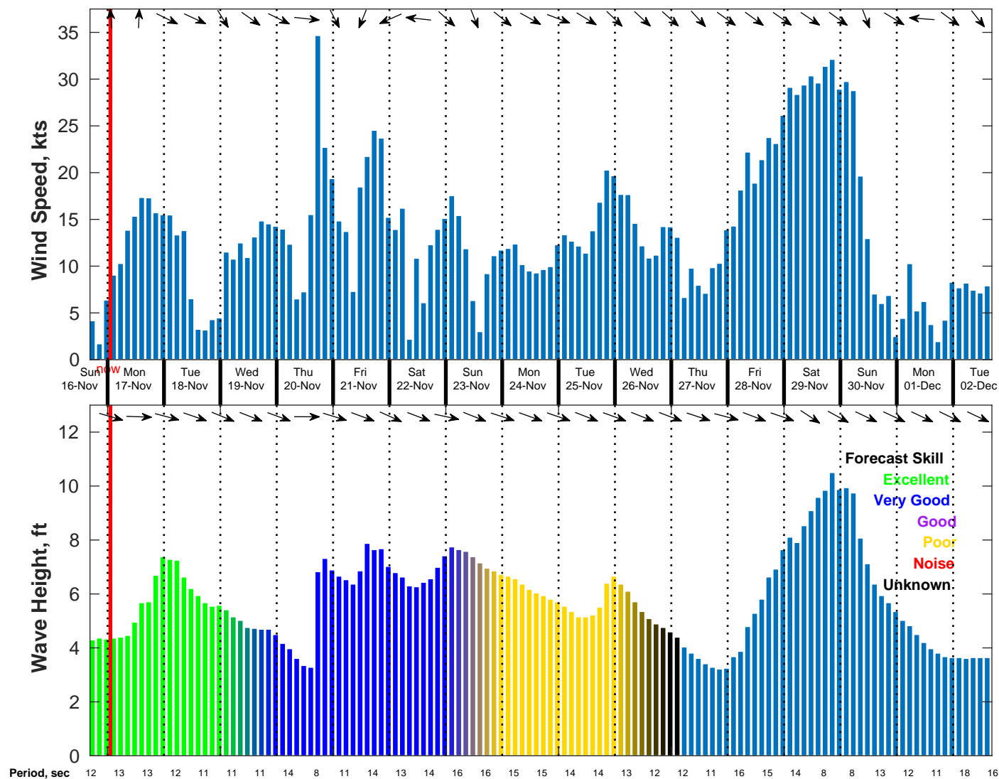
Wind & Wave Forecast for NDBC 46069 from 16-Nov-2025 16:00:00 to 02-Dec-2025 16:00:00
