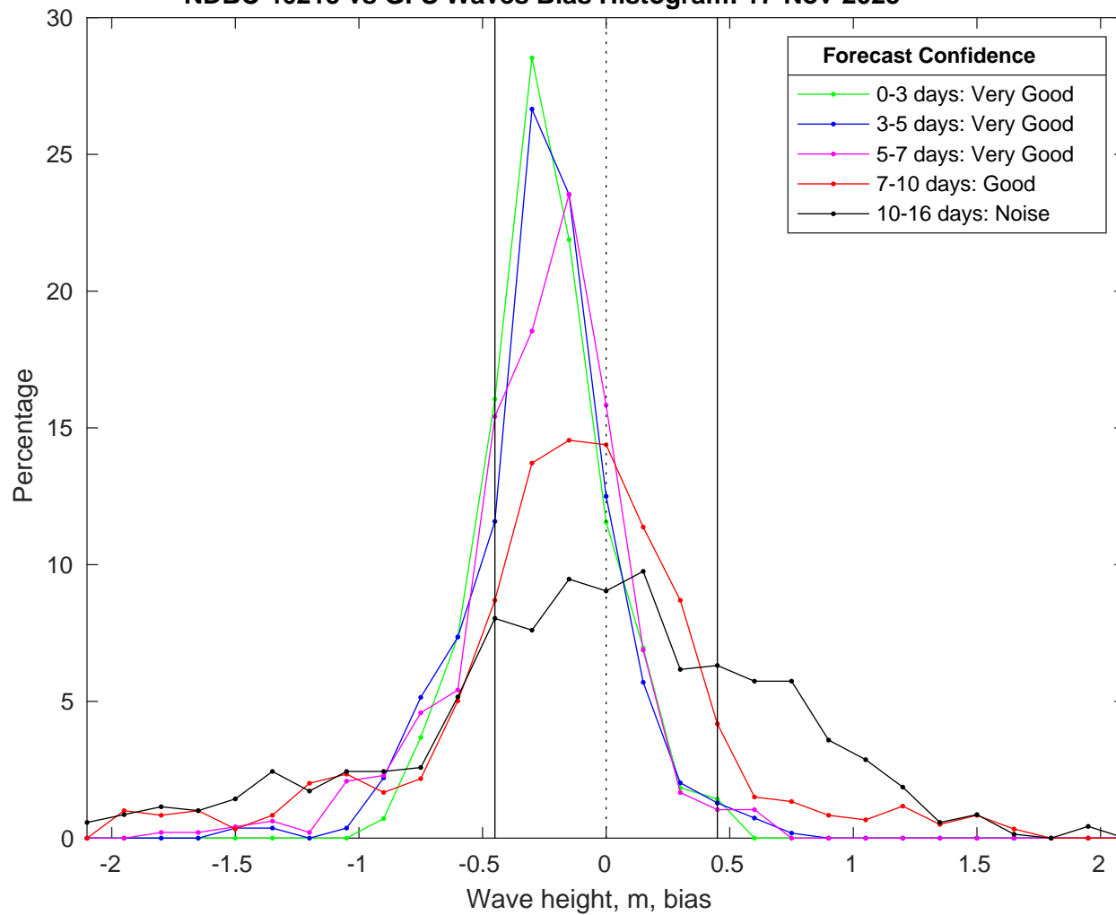
NDBC 46215 vs GFS Waves Bias Histogram: 17-Nov-2025
