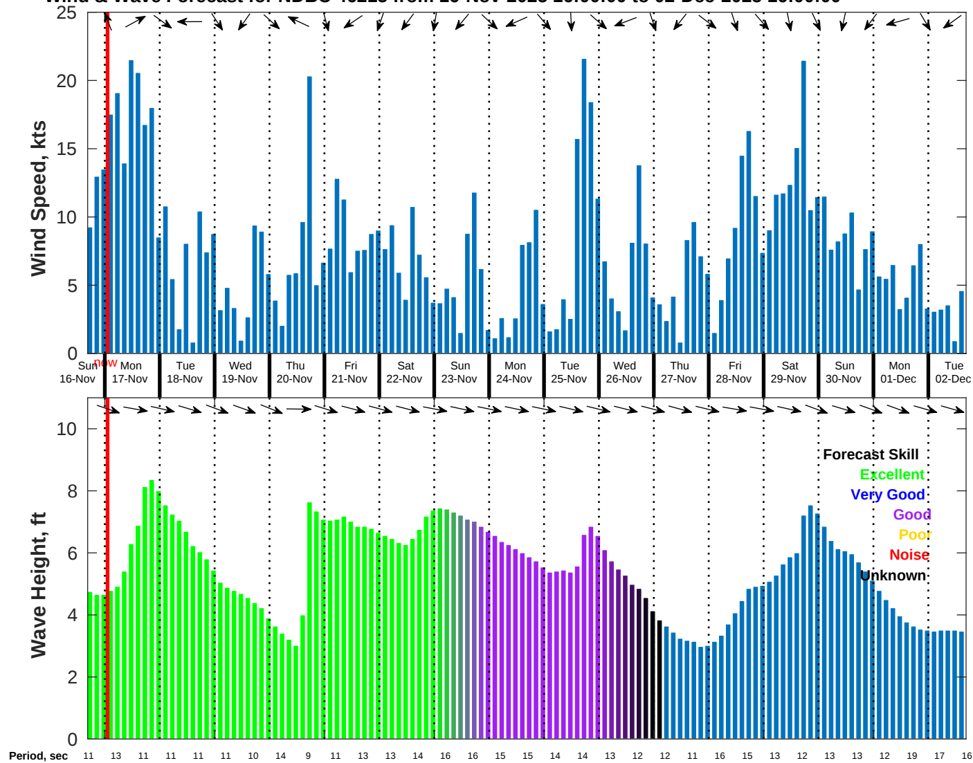
Wind & Wave Forecast for NDBC 46215 from 16-Nov-2025 16:00:00 to 02-Dec-2025 16:00:00
