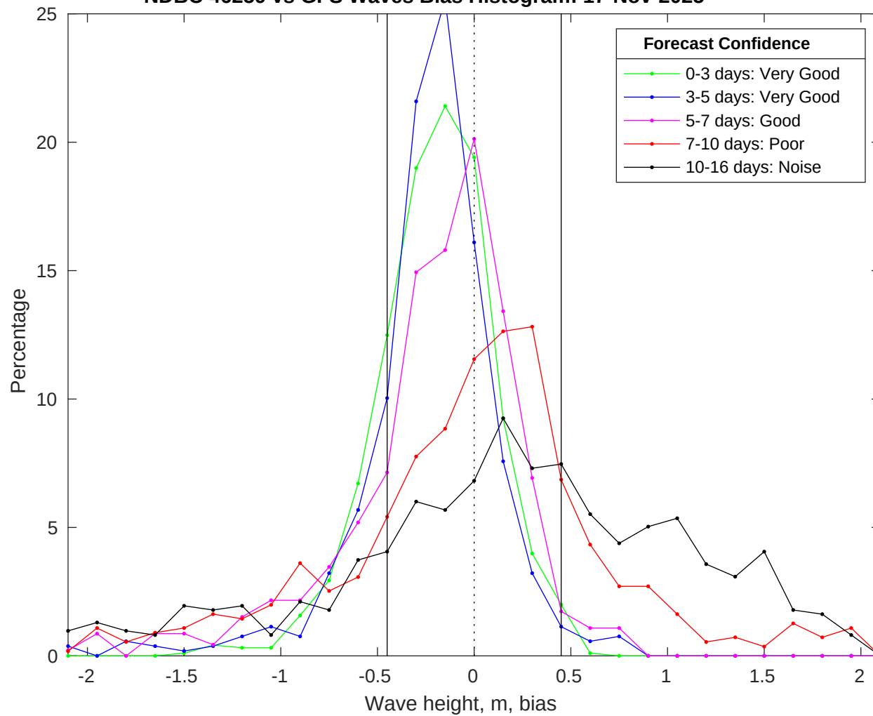
NDBC 46259 vs GFS Waves Bias Histogram: 17-Nov-2025
