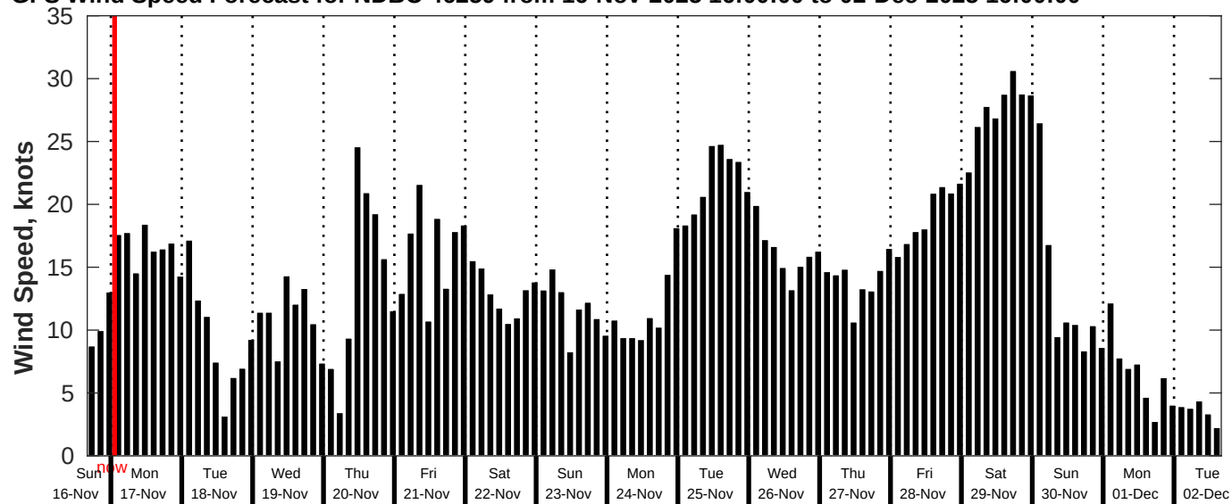
GFS Wind Speed Forecast for NDBC 46259 from 16-Nov-2025 16:00:00 to 02-Dec-2025 16:00:00
