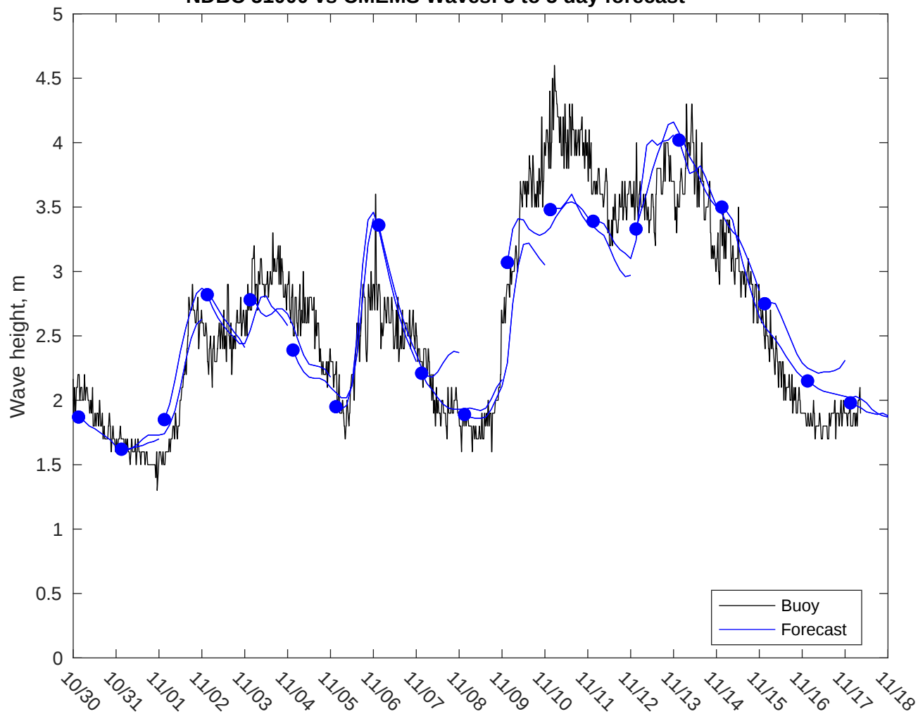
NDBC 51000 vs CMEMS Waves: 3 to 5 day forecast
