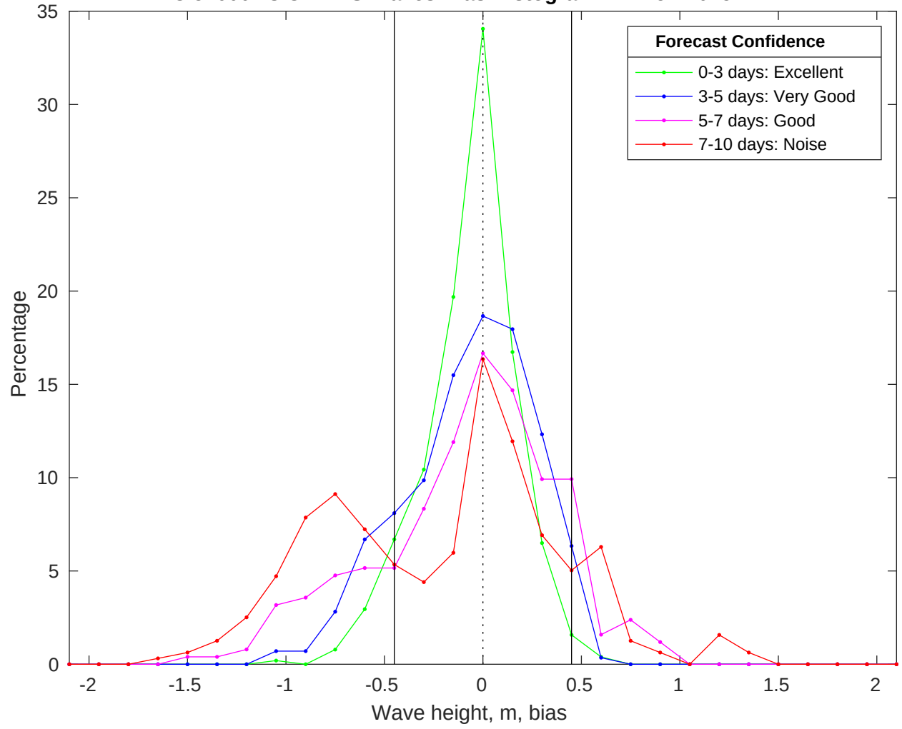
NDBC 51000 vs CMEMS Waves Bias Histogram: 17-Nov-2025
