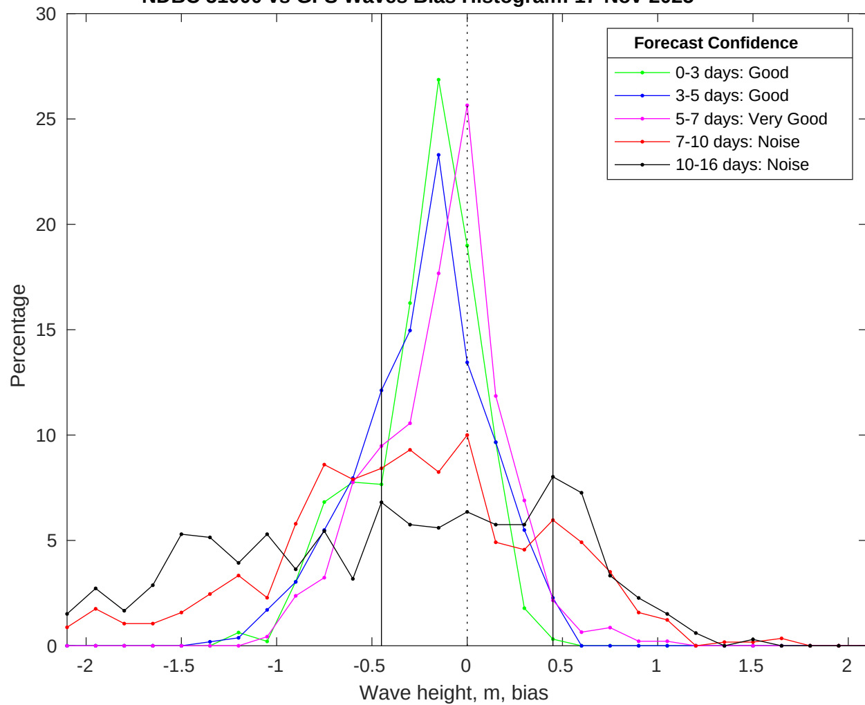
NDBC 51000 vs GFS Waves Bias Histogram: 17-Nov-2025
