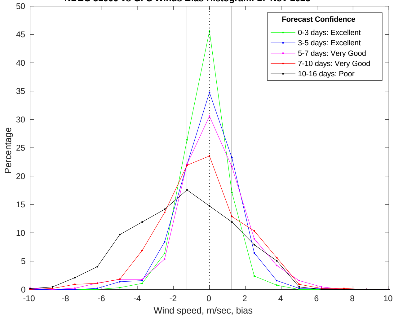
NDBC 51000 vs GFS Winds Bias Histogram: 17-Nov-2025
