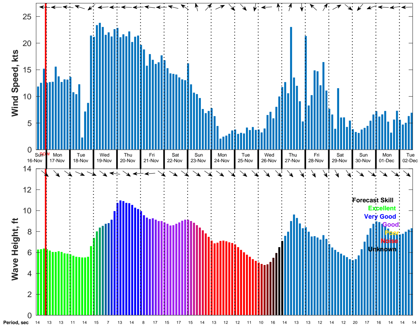
Wind & Wave Forecast for NDBC 51000 from 16-Nov-2025 14:00:00 to 02-Dec-2025 14:00:00
