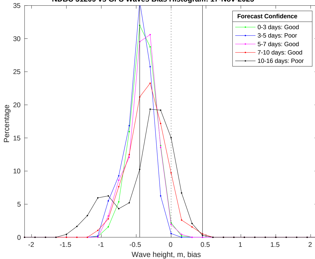
NDBC 51209 vs GFS Waves Bias Histogram: 17-Nov-2025
