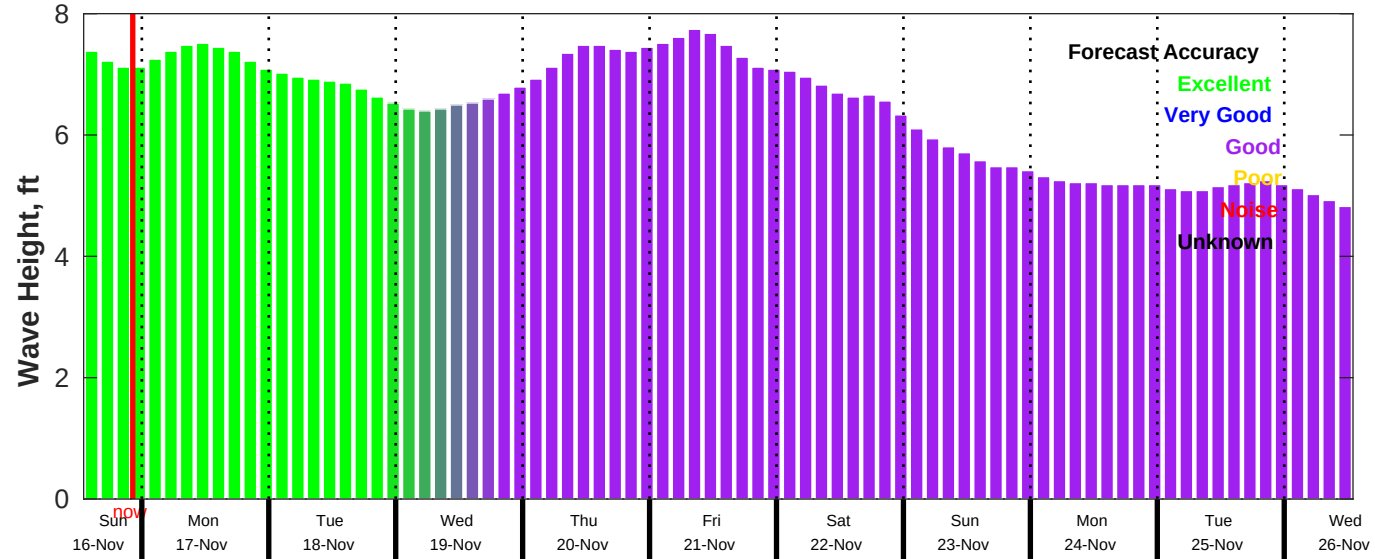
CMEMS Wave Forecast for NDBC 51209 from 16-Nov-2025 13:00:00 to 26-Nov-2025 13:00:00
