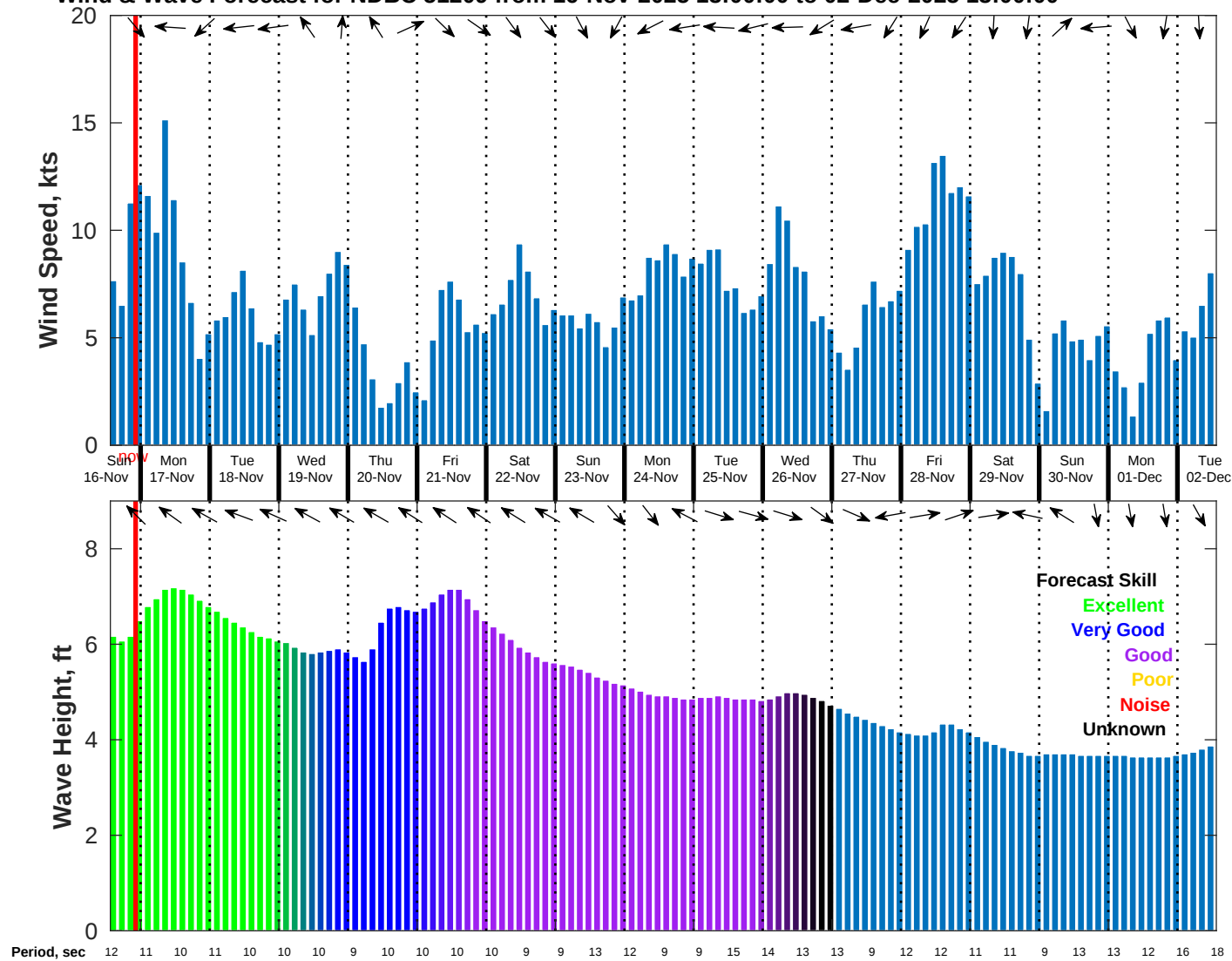
Wind & Wave Forecast for NDBC 51209 from 16-Nov-2025 13:00:00 to 02-Dec-2025 13:00:00
