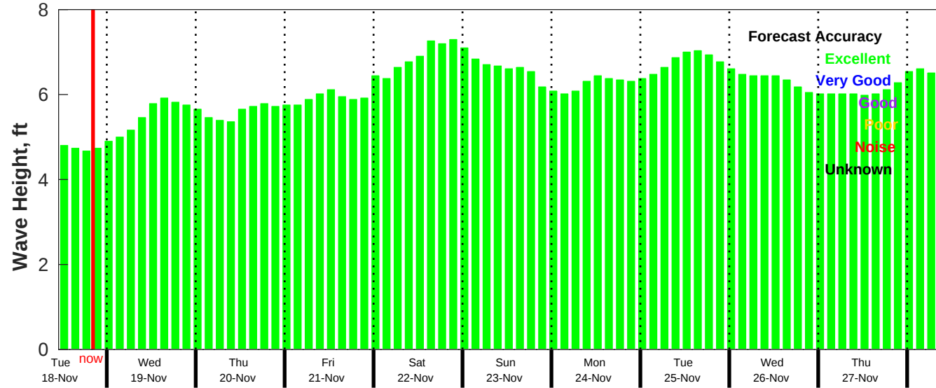
CMEMS Wave Forecast for NDBC 52211 from 17-Nov-2025 11:00:00 to 27-Nov-2025 11:00:00
