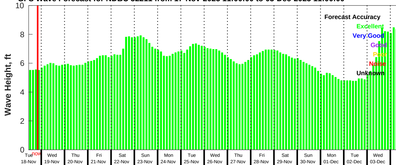
GFS Wave Forecast for NDBC 52211 from 17-Nov-2025 11:00:00 to 03-Dec-2025 11:00:00
