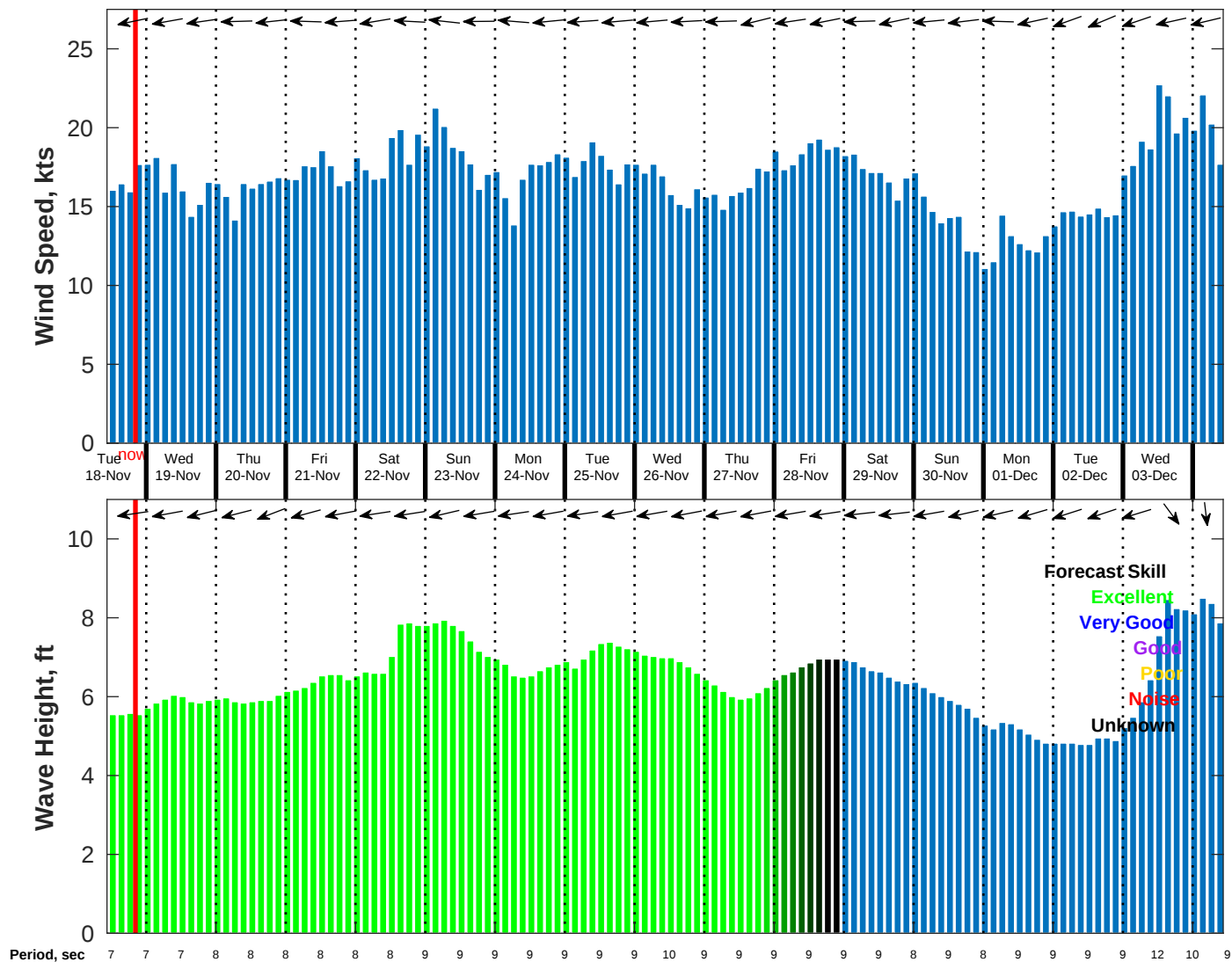
Wind & Wave Forecast for NDBC 52211 from 17-Nov-2025 11:00:00 to 03-Dec-2025 11:00:00
