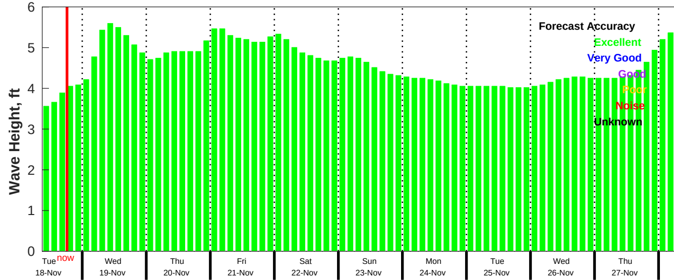
CMEMS Wave Forecast for NDBC 52212 from 17-Nov-2025 09:00:00 to 27-Nov-2025 09:00:00
