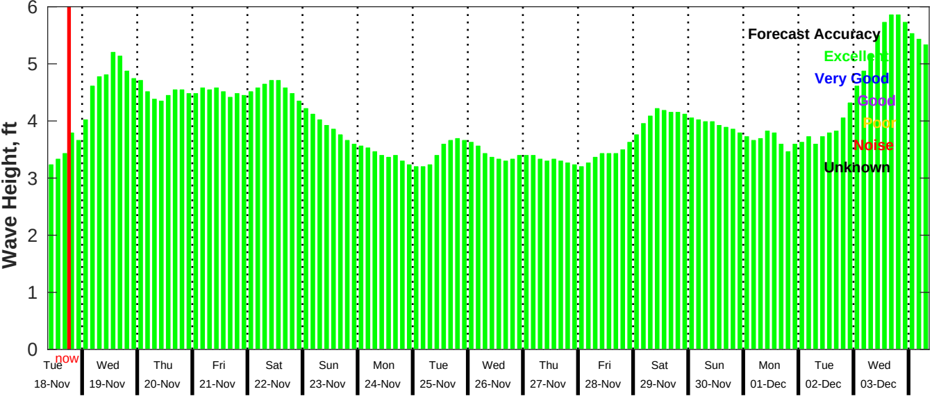
GFS Wave Forecast for NDBC 52212 from 17-Nov-2025 09:00:00 to 03-Dec-2025 09:00:00
