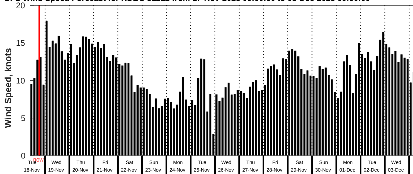
GFS Wind Speed Forecast for NDBC 52212 from 17-Nov-2025 09:00:00 to 03-Dec-2025 09:00:00
