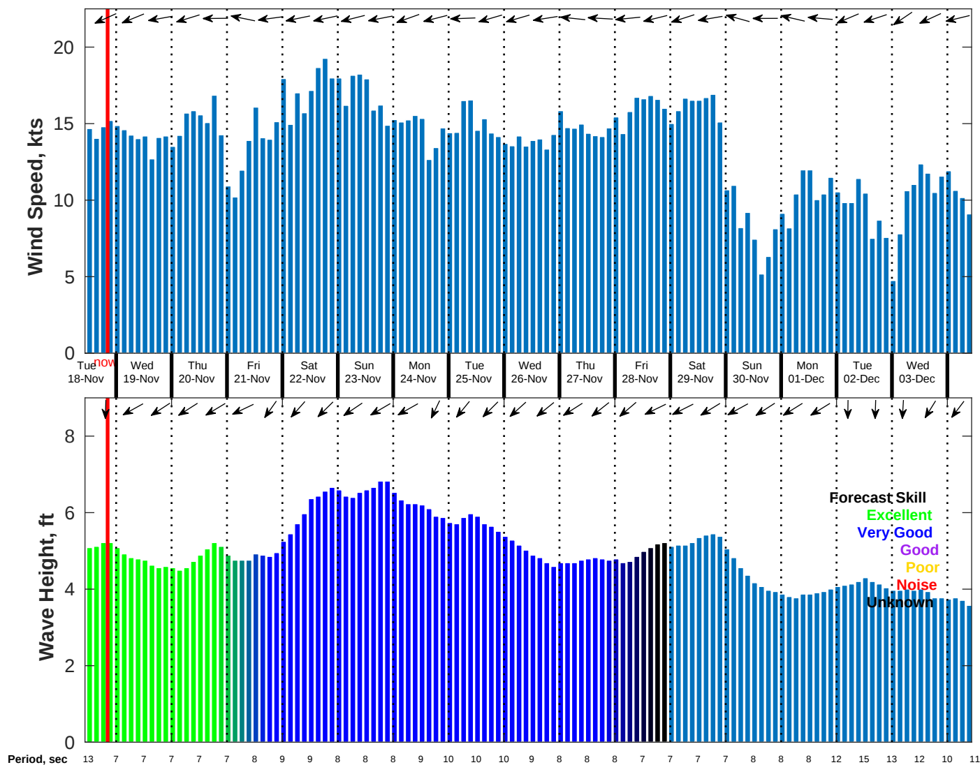
Wind & Wave Forecast for NDBC 52213 from 17-Nov-2025 11:00:00 to 03-Dec-2025 11:00:00
