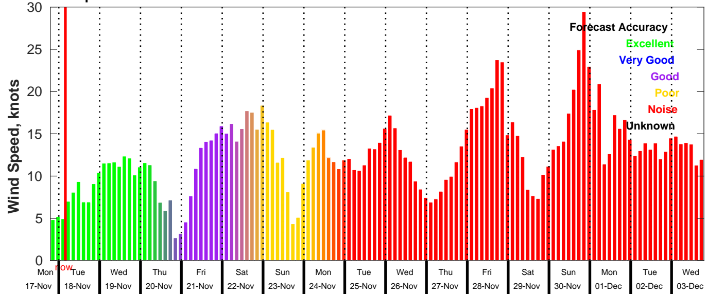
GFS Wind Speed Forecast for NDBC 41004 from 17-Nov-2025 19:00:00 to 03-Dec-2025 19:00:00
