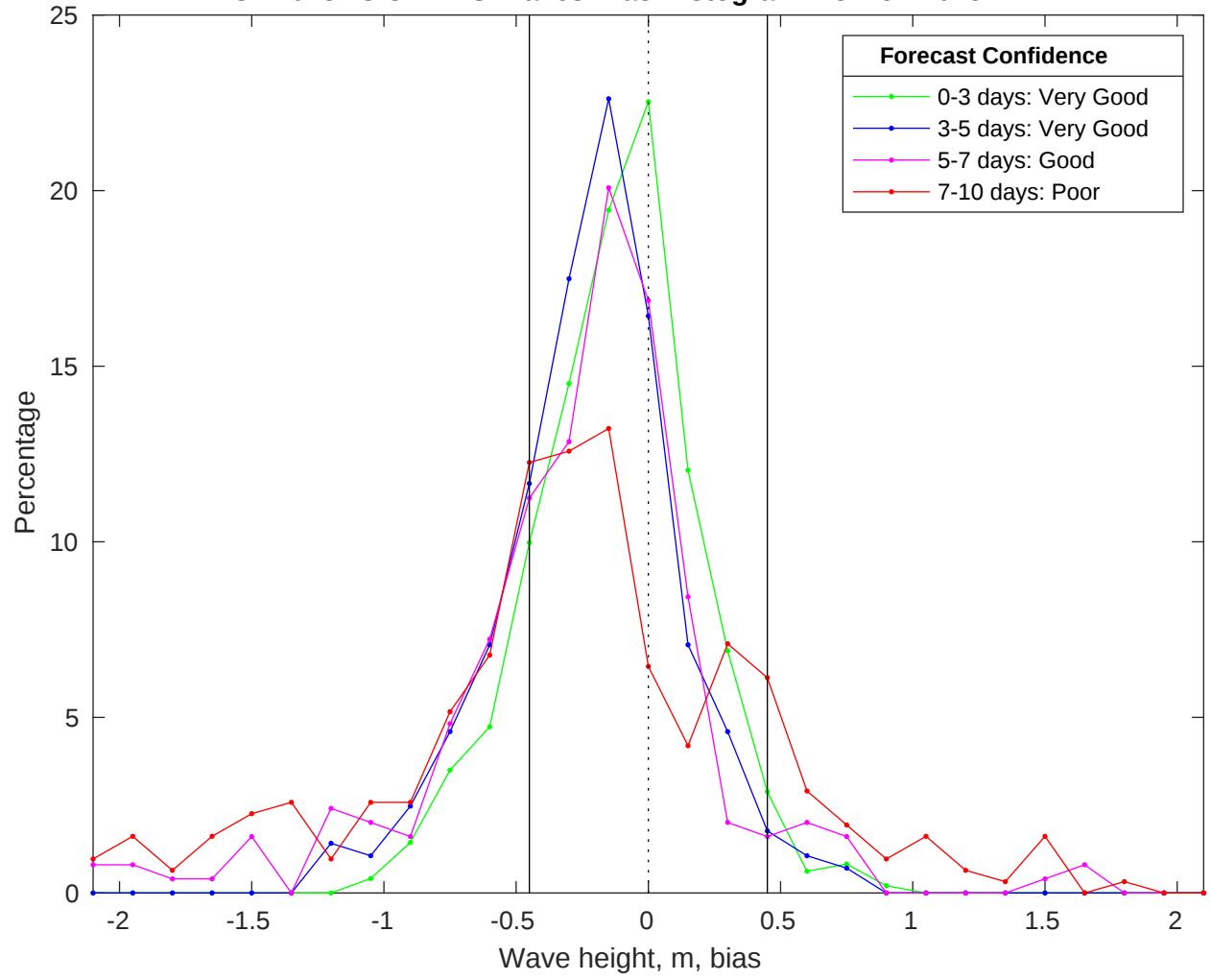
NDBC 41013 vs CMEMS Waves Bias Histogram: 18-Nov-2025
