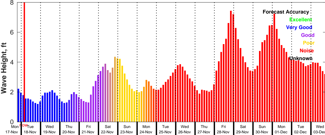
GFS Wave Forecast for NDBC 41013 from 17-Nov-2025 19:00:00 to 03-Dec-2025 19:00:00
