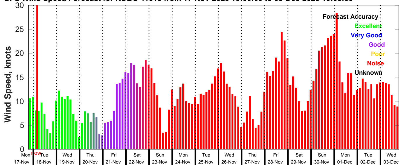
GFS Wind Speed Forecast for NDBC 41013 from 17-Nov-2025 19:00:00 to 03-Dec-2025 19:00:00
