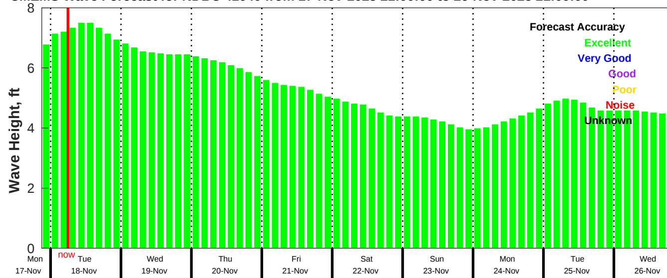
CMEMS Wave Forecast for NDBC 41040 from 17-Nov-2025 21:00:00 to 26-Nov-2025 21:00:00
