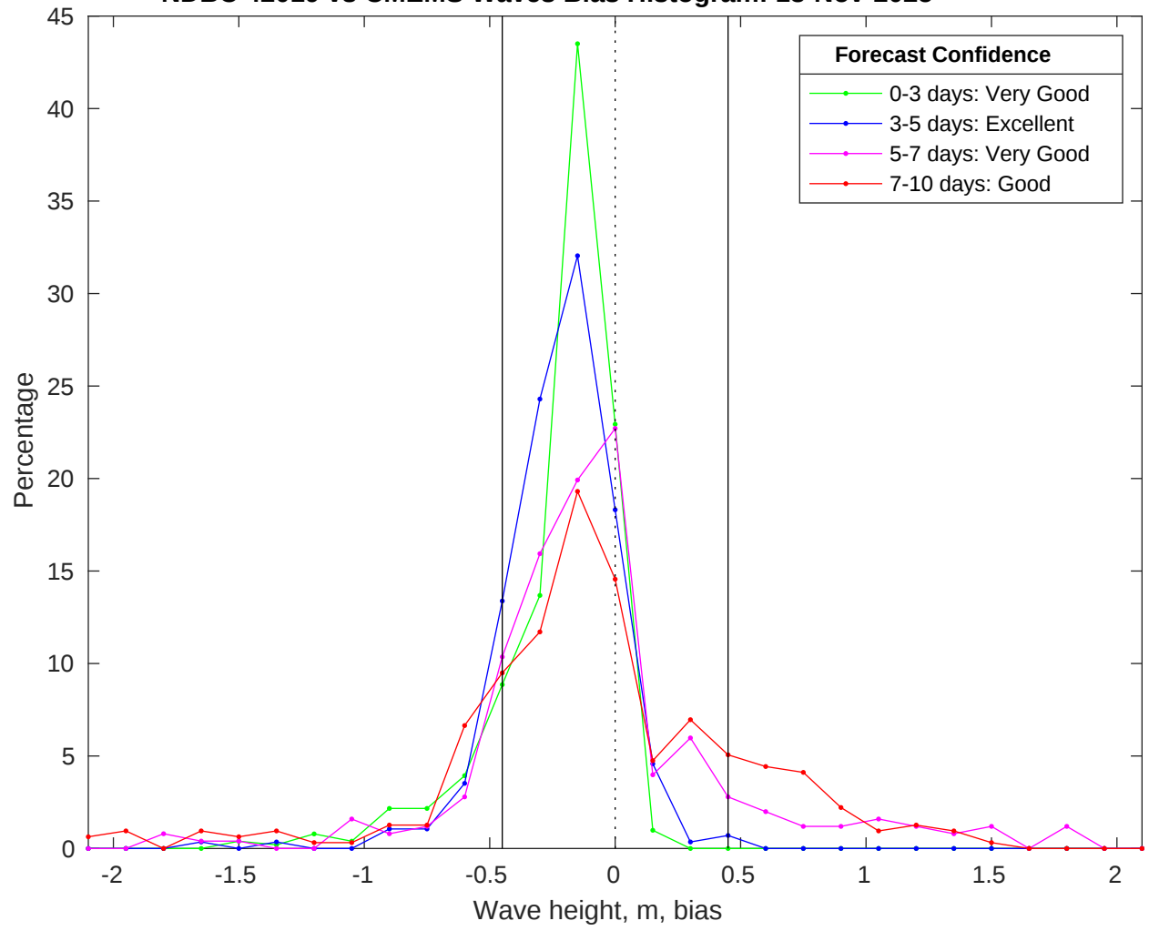
NDBC 42019 vs CMEMS Waves Bias Histogram: 18-Nov-2025
