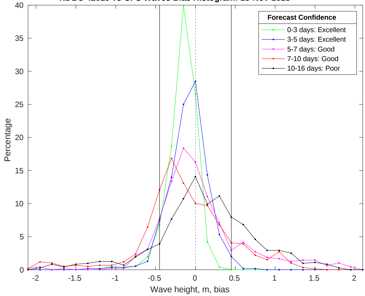
NDBC 42019 vs GFS Waves Bias Histogram: 18-Nov-2025
