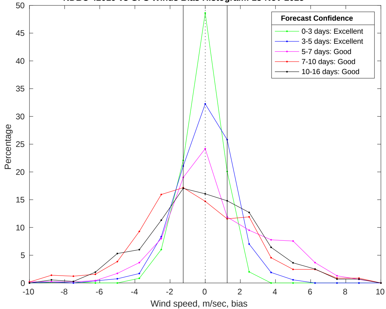
NDBC 42019 vs GFS Winds Bias Histogram: 18-Nov-2025
