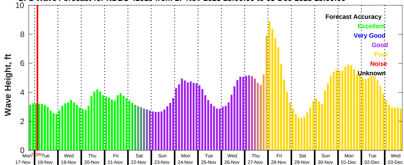
GFS Wave Forecast for NDBC 42019 from 17-Nov-2025 18:00:00 to 03-Dec-2025 18:00:00
