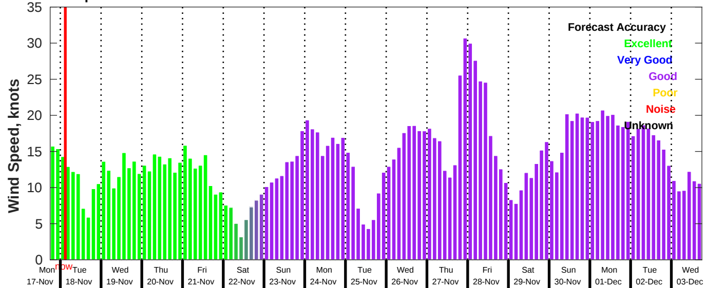
GFS Wind Speed Forecast for NDBC 42019 from 17-Nov-2025 18:00:00 to 03-Dec-2025 18:00:00
