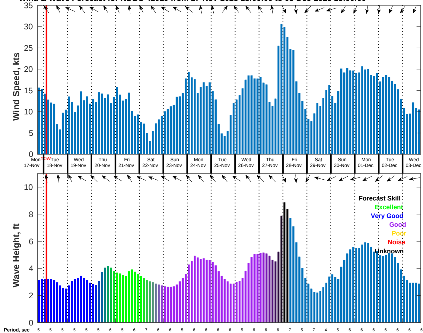
Wind & Wave Forecast for NDBC 42019 from 17-Nov-2025 18:00:00 to 03-Dec-2025 18:00:00
