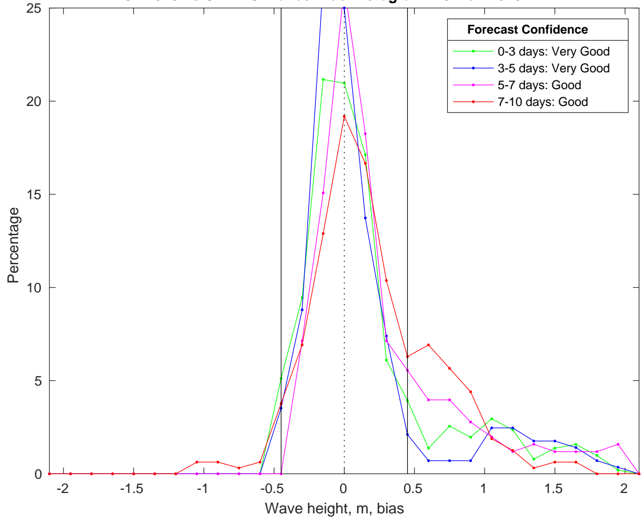
NDBC 42020 vs CMEMS Waves Bias Histogram: 18-Nov-2025
