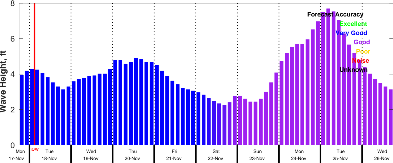
CMEMS Wave Forecast for NDBC 42020 from 17-Nov-2025 18:00:00 to 26-Nov-2025 18:00:00
