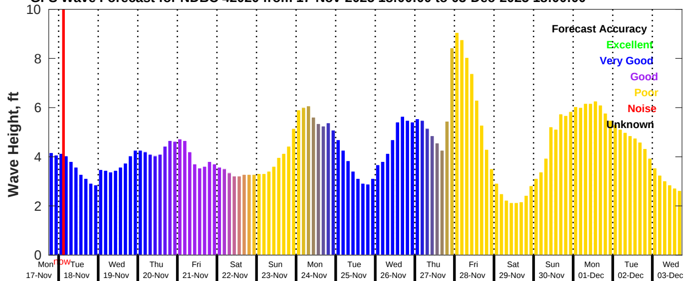
GFS Wave Forecast for NDBC 42020 from 17-Nov-2025 18:00:00 to 03-Dec-2025 18:00:00
