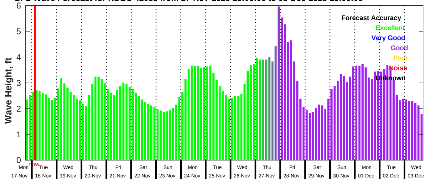
GFS Wave Forecast for NDBC 42035 from 17-Nov-2025 18:00:00 to 03-Dec-2025 18:00:00
