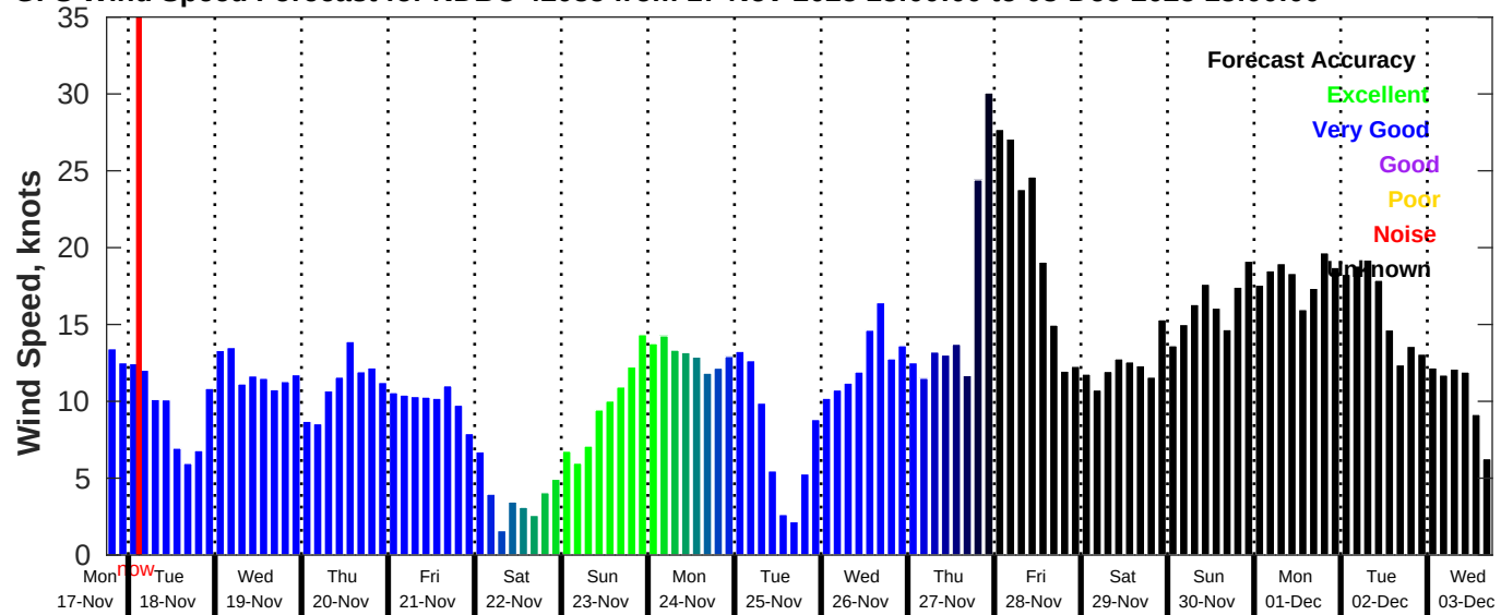
GFS Wind Speed Forecast for NDBC 42035 from 17-Nov-2025 18:00:00 to 03-Dec-2025 18:00:00
