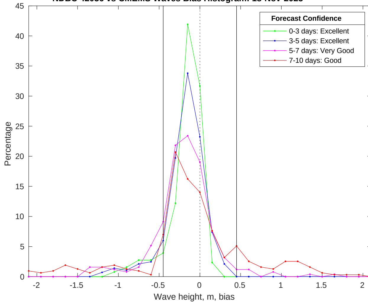
NDBC 42036 vs CMEMS Waves Bias Histogram: 18-Nov-2025
