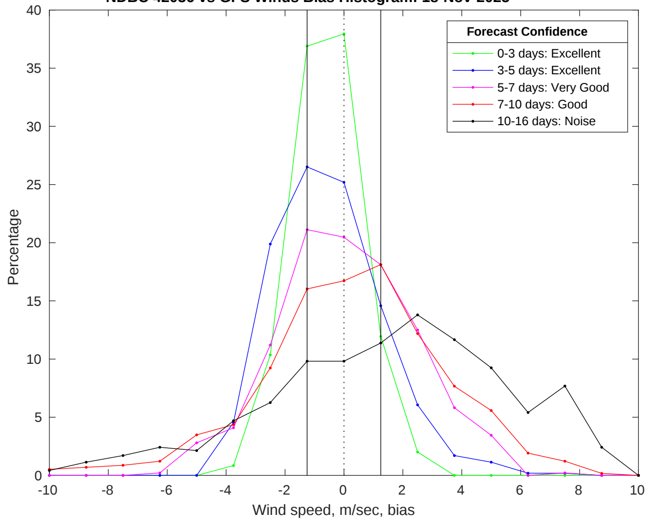
NDBC 42036 vs GFS Winds Bias Histogram: 18-Nov-2025
