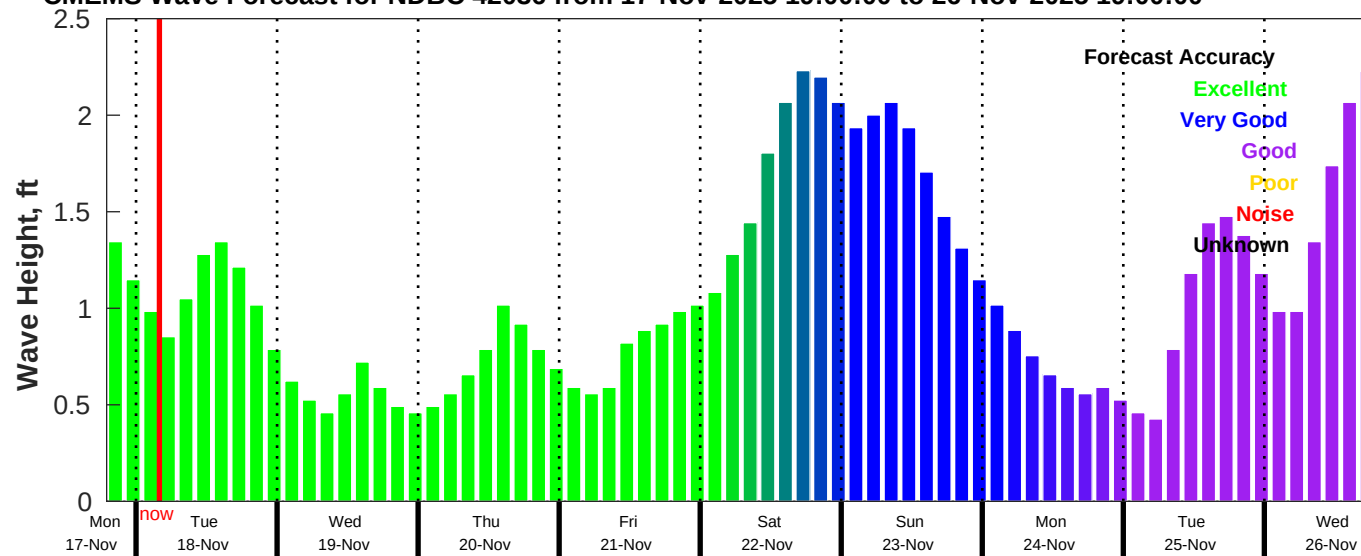
CMEMS Wave Forecast for NDBC 42036 from 17-Nov-2025 19:00:00 to 26-Nov-2025 19:00:00
