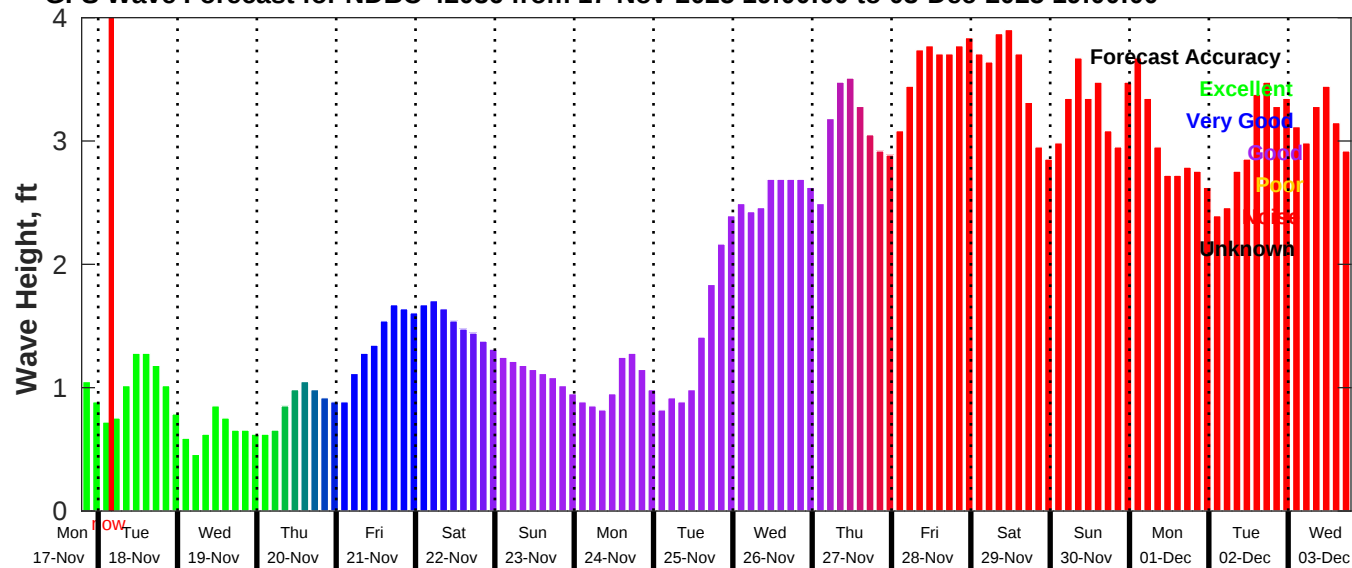
GFS Wave Forecast for NDBC 42036 from 17-Nov-2025 19:00:00 to 03-Dec-2025 19:00:00
