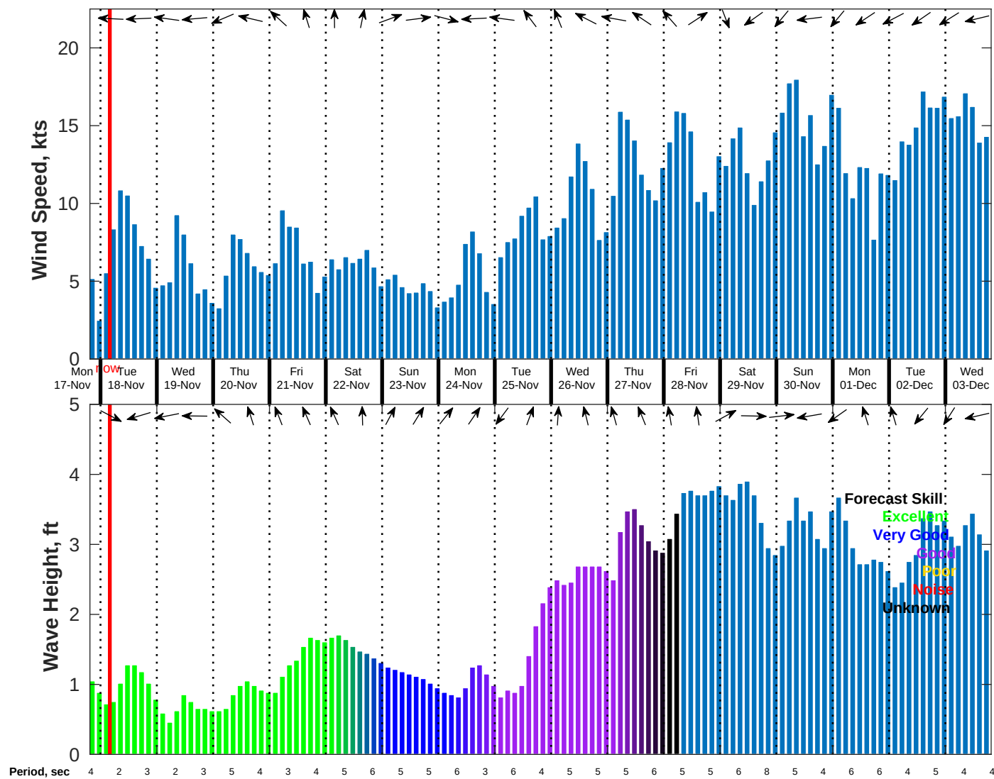
Wind & Wave Forecast for NDBC 42036 from 17-Nov-2025 19:00:00 to 03-Dec-2025 19:00:00
