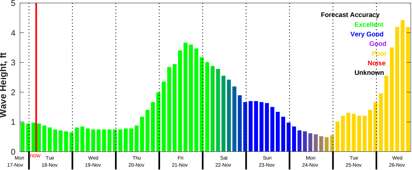
CMEMS Wave Forecast for NDBC 42040 from 17-Nov-2025 19:00:00 to 26-Nov-2025 19:00:00
